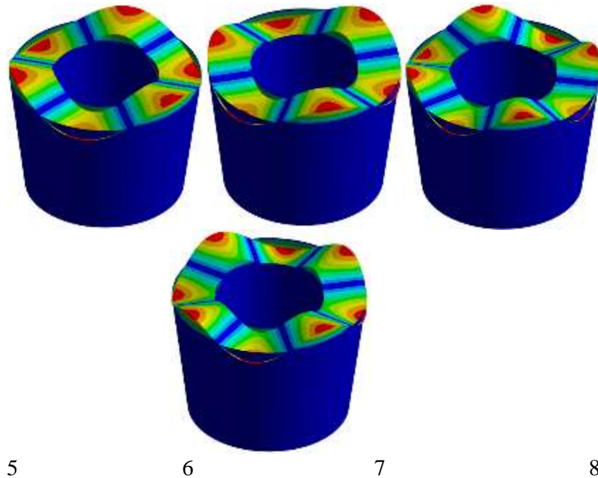
Fig.2. Sloshing Modes of Structure
