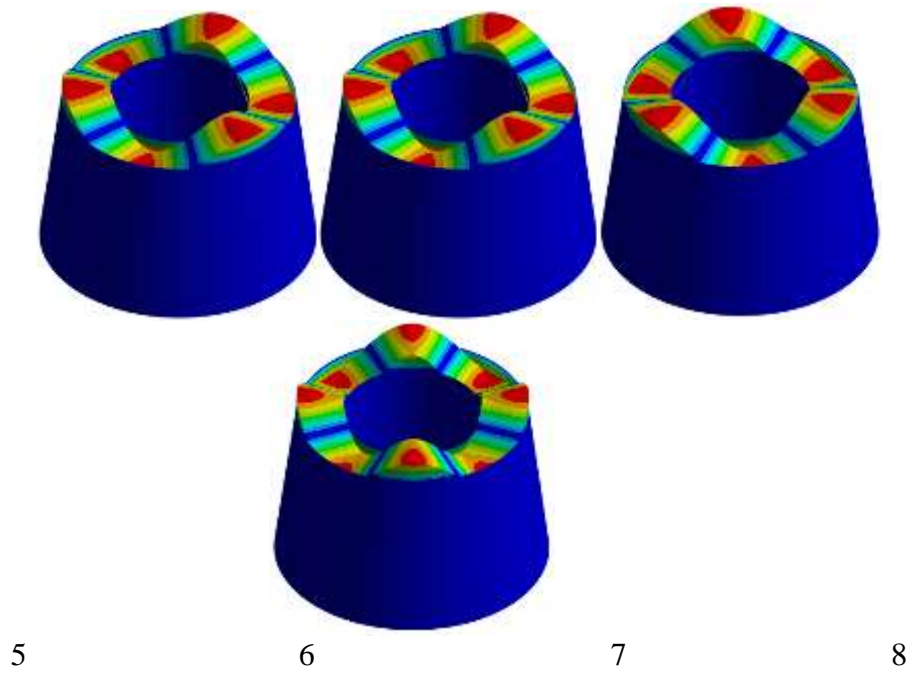
Fig. 1. Sloshing Modes of Structure.
